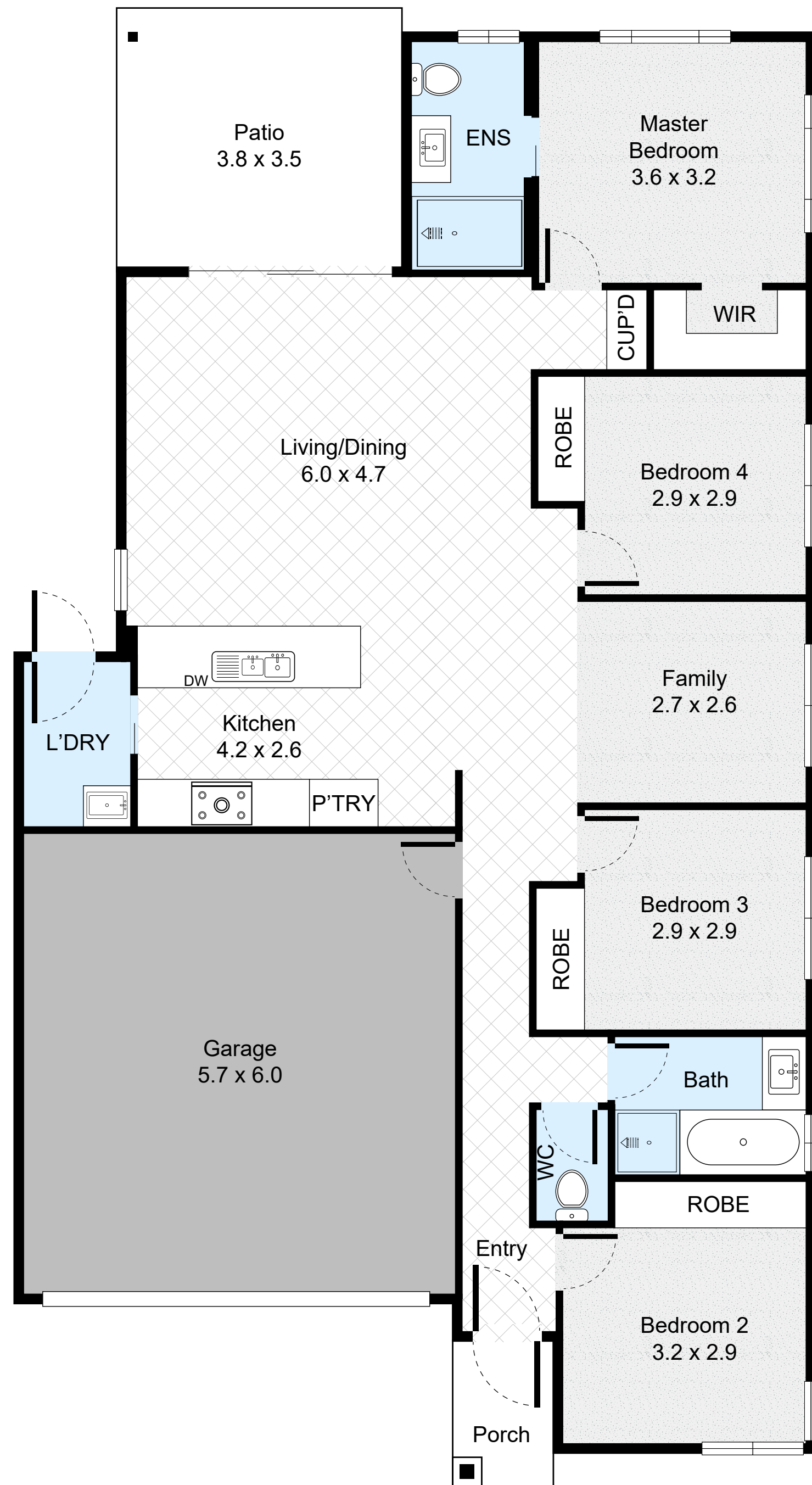
FLOOR PLAN
