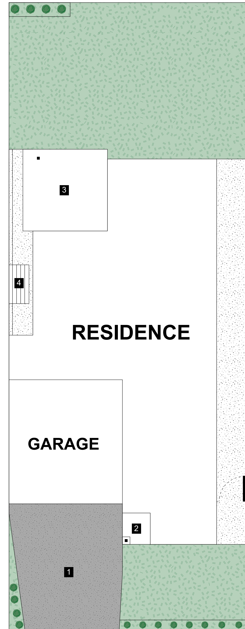
SITE PLAN
