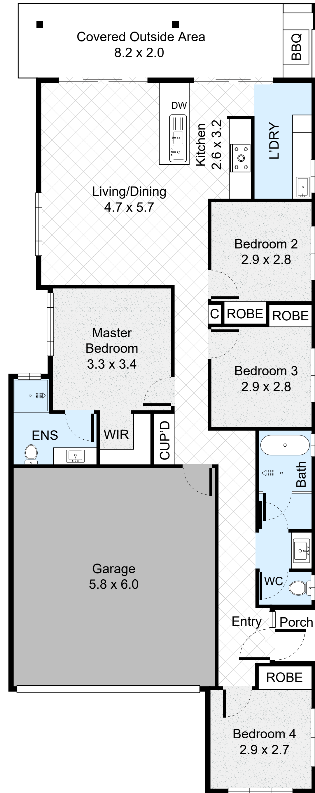
FLOOR PLAN
